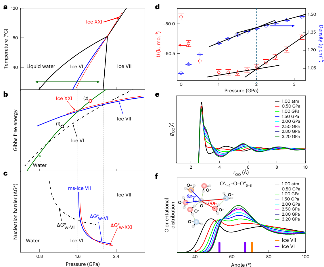
Fig. 4 | Phase stability of ice phases and MD simulation results. a , Phase diagram of \text{H}_2\text{O} . b, c , Schematic of the Gibbs free energy ( b ) and nucleation barriers ( c ) for the four phases of water, ice VI, ms-ice VII and ms-ice XXI. The red lines in a–c denote the ice XXI phase, which are presumed, based on experimental observations (see details in the main text). d–f , Simulation results of SW are obtained using the SPCfw potential. d , Potential energy and density versus
