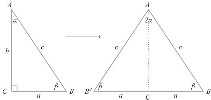
Figure 7. Creating \triangle ABB' .
